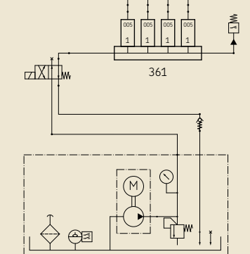
Hydraulic layout
